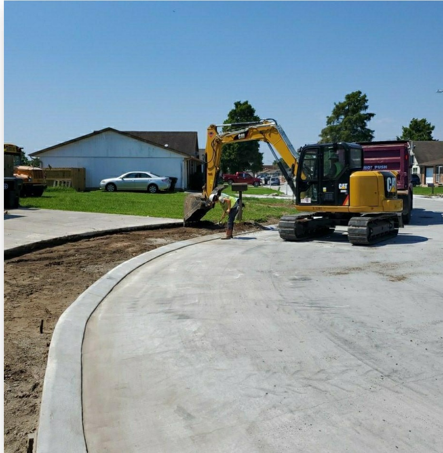
An example of newly paved block on the Village De L'Est Group B project.
